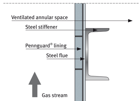
Figure 2 With an insulating Pennguard® lining on the inside of the flue, outside stiffeners can no longer lead to cold spots.
